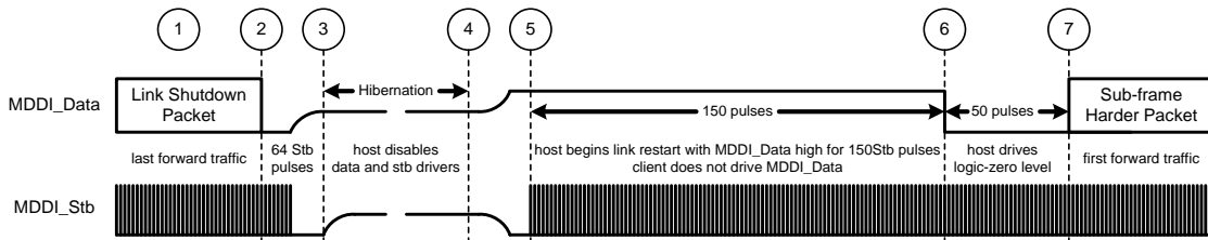
Figure 64. Host-initiated Link Wake-up Sequence
