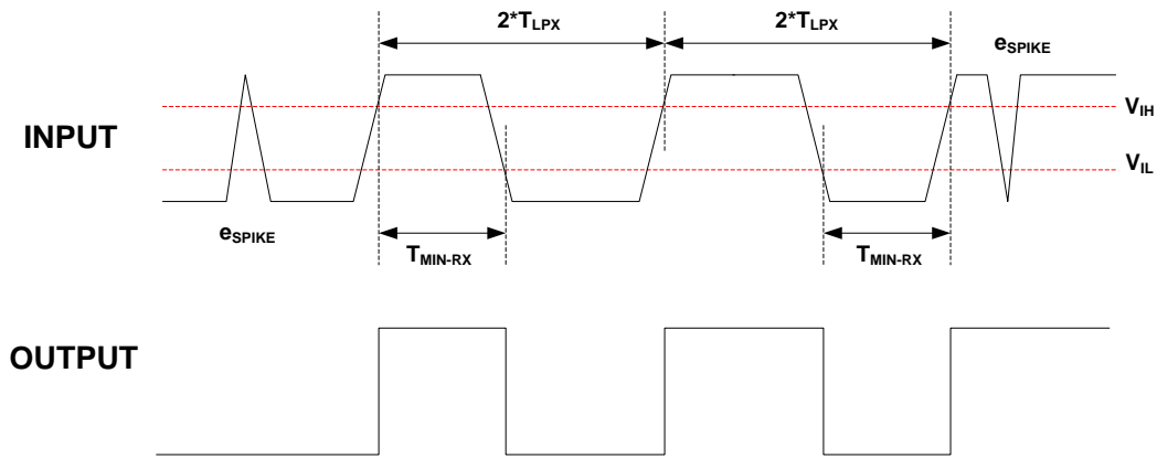
Figure 104. AC Timing Waveform for LP Mode MIPI Operation
