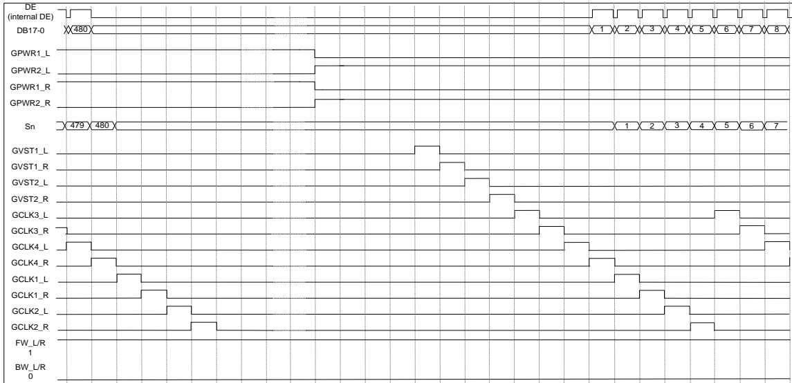
Figure 90. Non-overlap, 8-phase, forward mode ( FHN=0, SDM=1, FV=0, FVST=0 )
