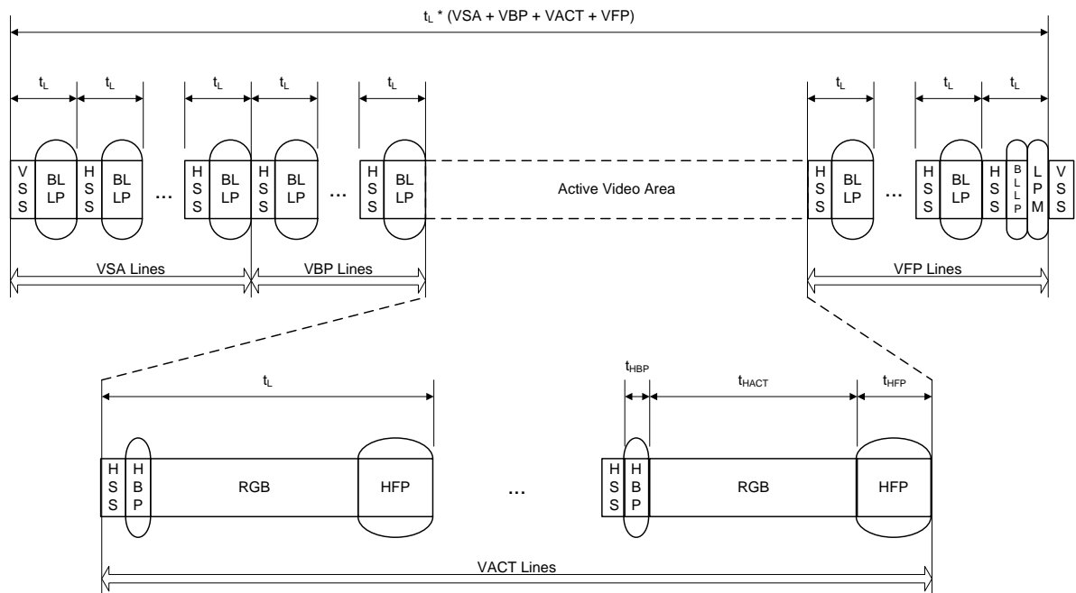
Figure 42. Non-Burst Mode with Sync Events
