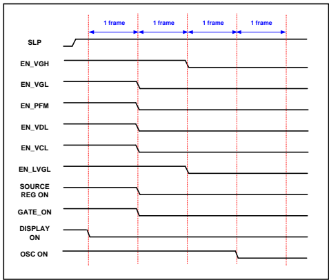
Power OFF STMODE[2:0]=2h
