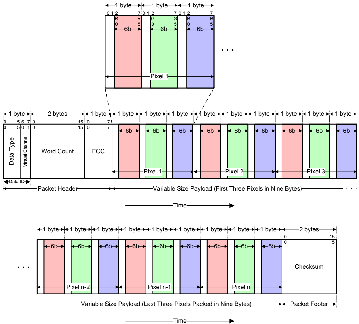
Figure 39. Loosely Packed Pixel Stream, 18-bit RGB, 6-6-6 Format
