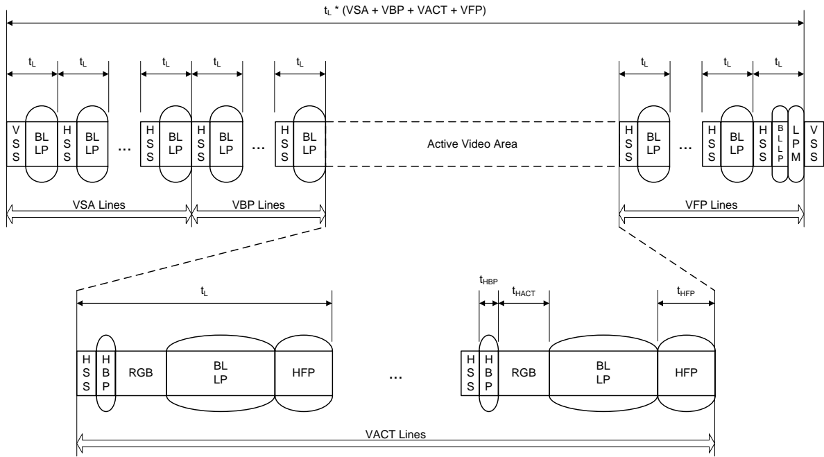
Figure 43. Burst mode
