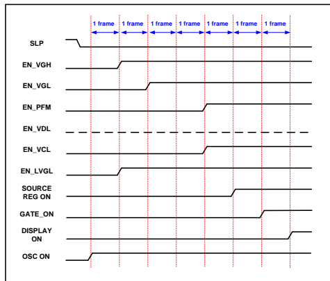
Power ON STMODE[2:0]=3h
