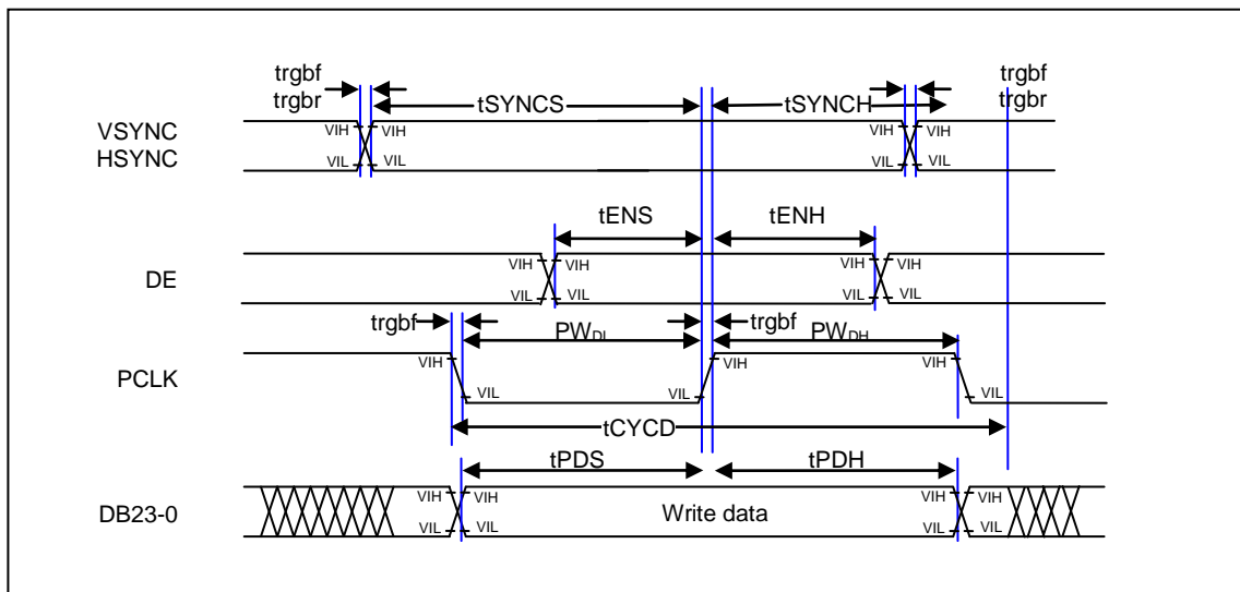
Figure 115. RGB interface
