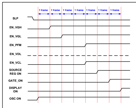
Power ON STMODE[2:0]=7h
