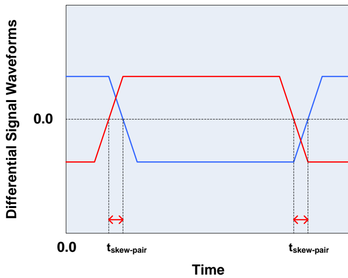
Figure 111. Interconnect Network skew between positive and negative outputs
