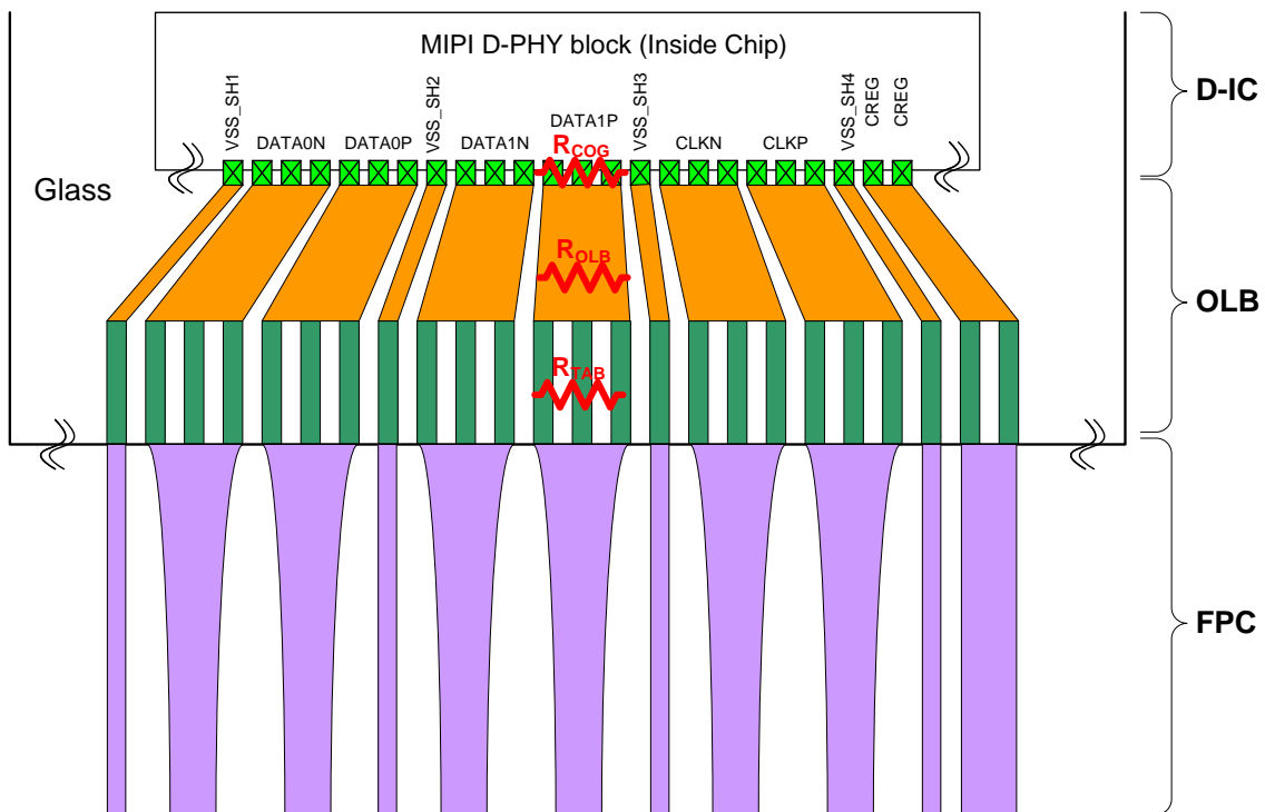
Figure 31. Consideration of the Resistance. R_{COG} + R_{OLB} + R_{FOB} < 10\text{ohm} . Assuming the other resistances of FPC patterns or connectors are negligibly small.
