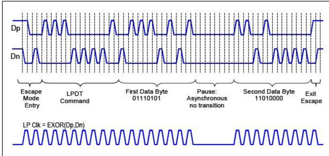
Figure 34. Low Power Data Transmission Sequence with D-PHY
