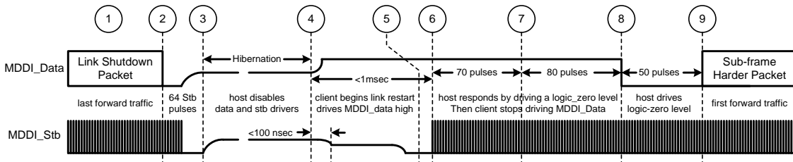
Figure 66. Client-initiated Link Wake-up Sequence
