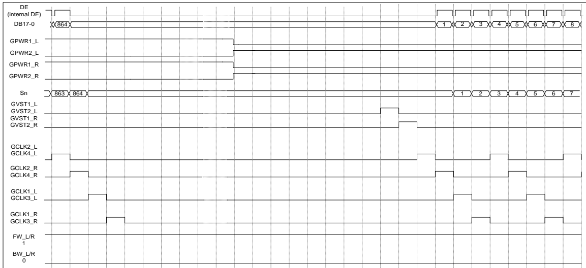
Figure 86. Non-overlap, 4-phase, forward mode ( FHN=0, SDM=0, FV=0, FVST=0 )
