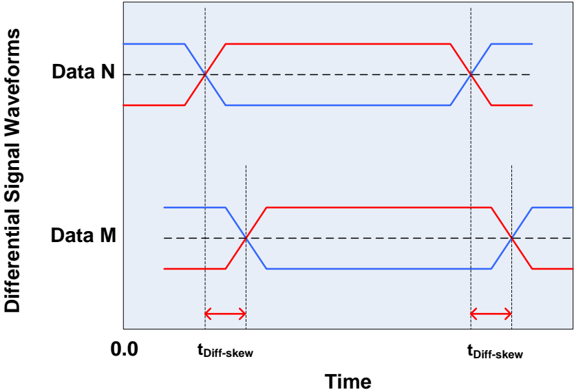
Figure 112. Interconnect Network peak delay skew between differential pairs
