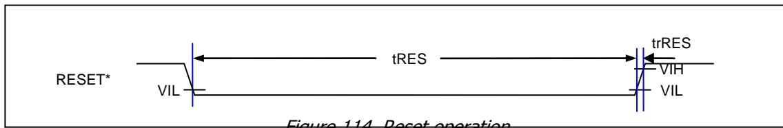
Figure 114. Reset operation
