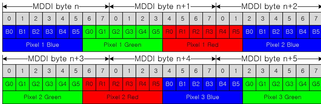
Figure 56. 18bits/pixel(B:6, G:6, R:6) data transfer format
