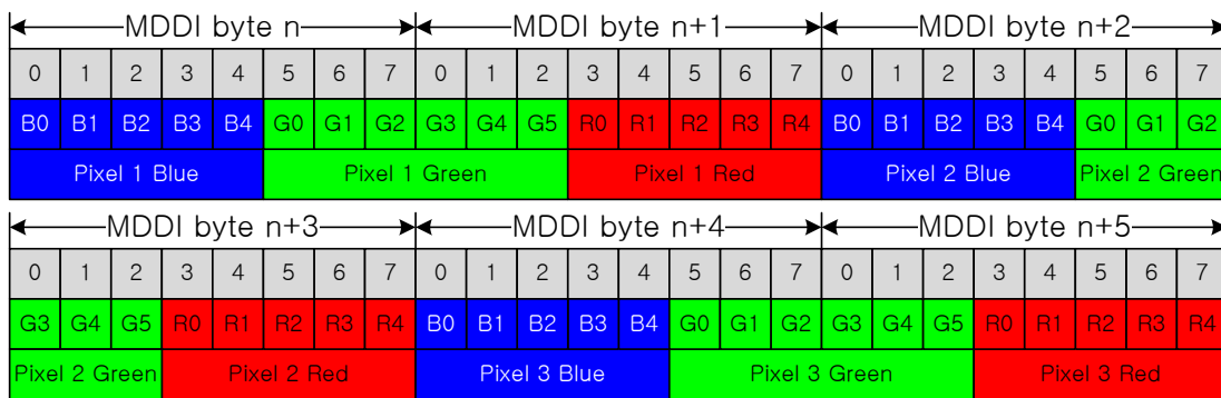
Figure 57. 16bits/pixel(B:5, G:6, R:5) data transfer format
