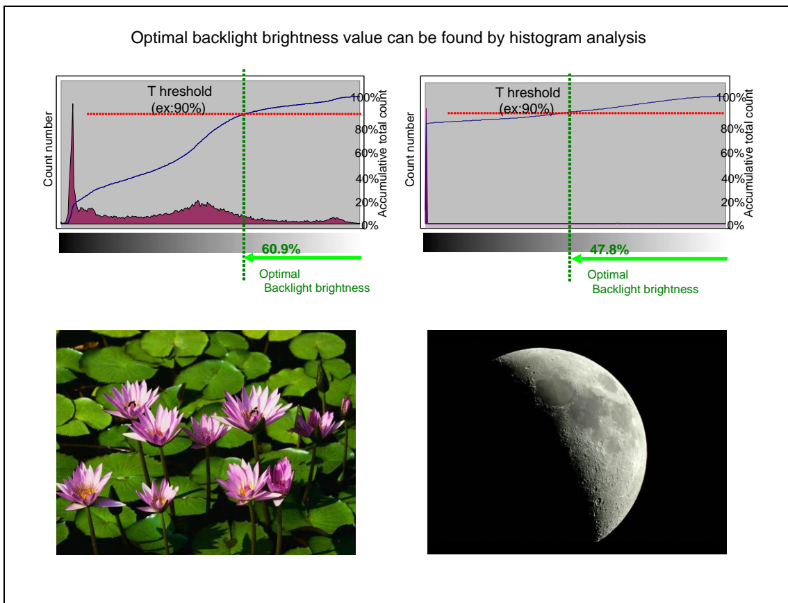
Figure 68. Content Adaptive Brightness Control
