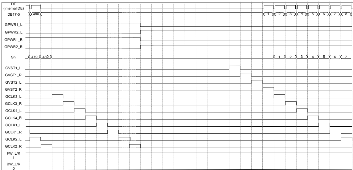
Figure 91. Non-overlap, 8-phase, forward, advanced DE mode ( FHN=0, SDM=1, FV=0, FVST=1 )
