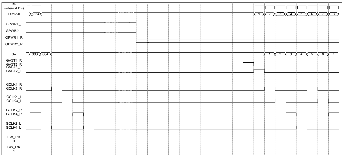
Figure 95. Non-overlap, 4-phase, backward, advanced DE mode ( FHN=0, SDM=0, FV=1, FVST=1 )
