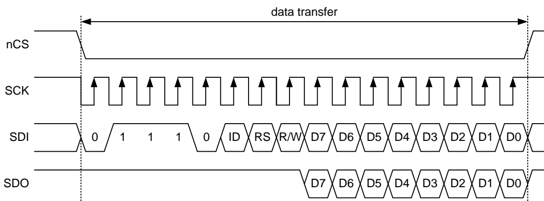
Figure 25. SPI Interface
