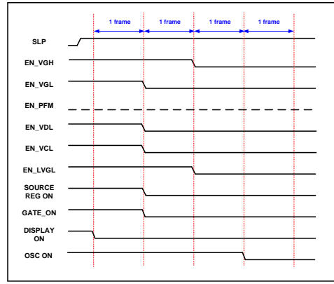
Power OFF STMODE[2:0]=1h
