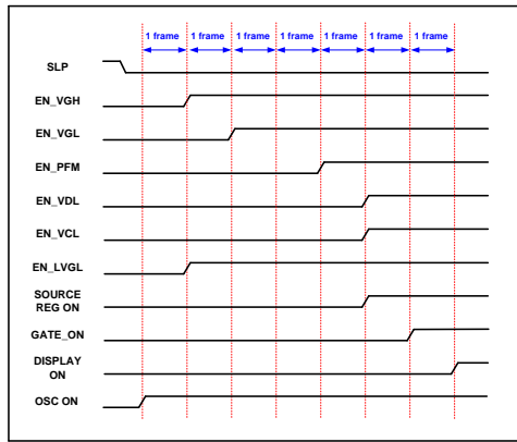
Power ON STMODE[2:0]=2h
