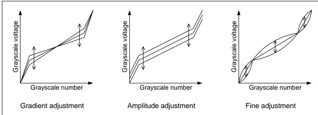
Figure 76. Gamma Adjustments
