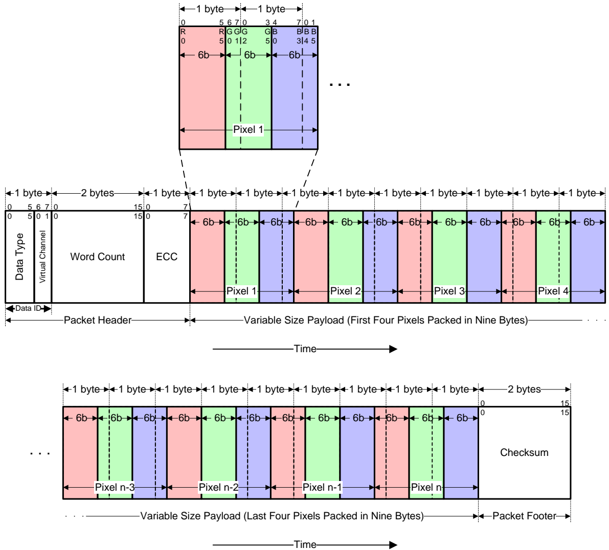
Figure 38. Packed Pixel Stream, 18-bit RGB, 6-6-6 Format
