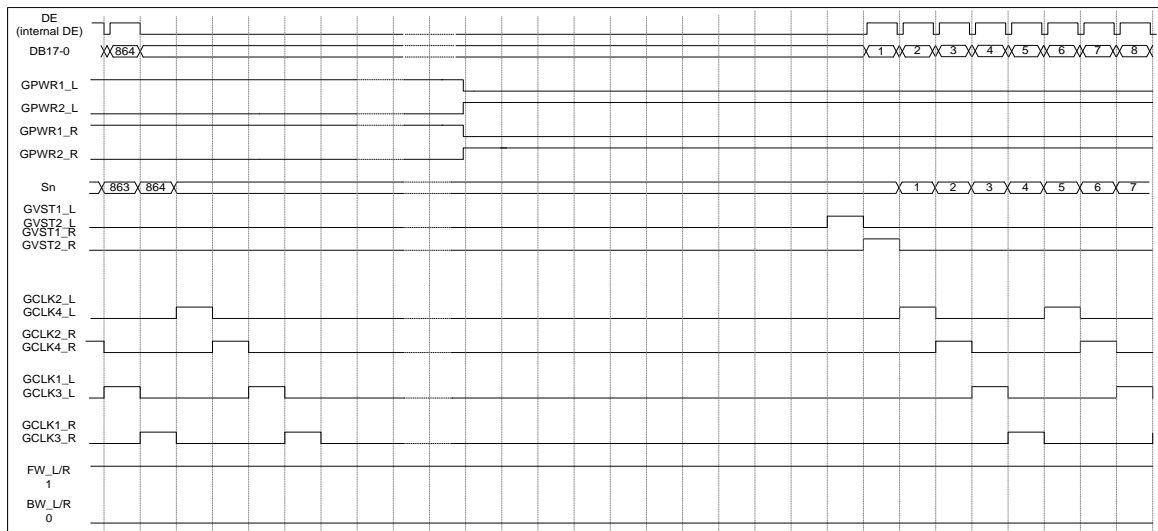
Figure 87. Non-overlap, 4-phase, forward, advanced DE mode ( FHN=0, SDM=0, FV=0, FVST=1 )
