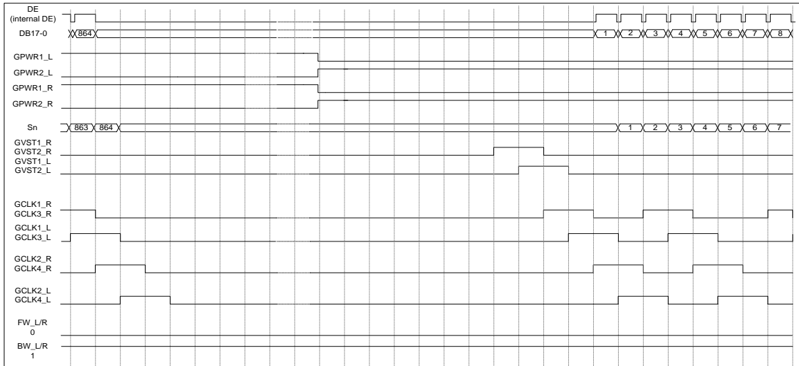
Figure 96. Overlap, 4-phase, backward mode ( FHN=1, SDM=0, FV=1, FVST=0 )
