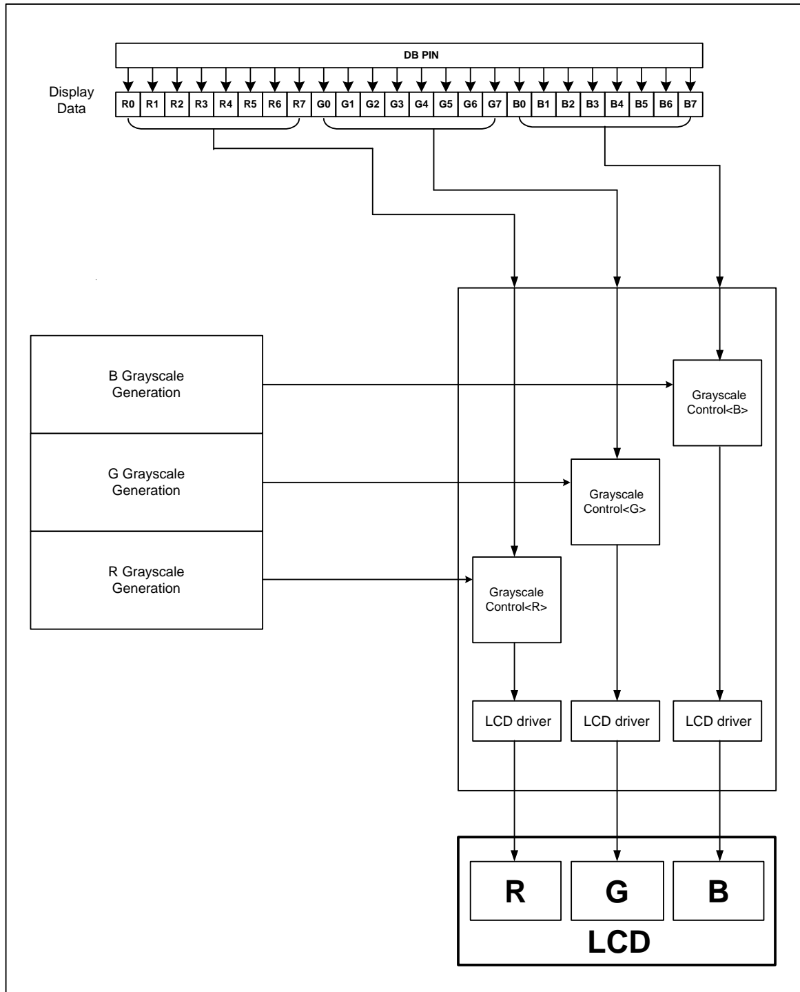
Figure 73. Grayscale Control
