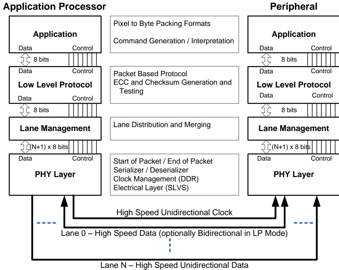
Figure 29. DSI Layers
