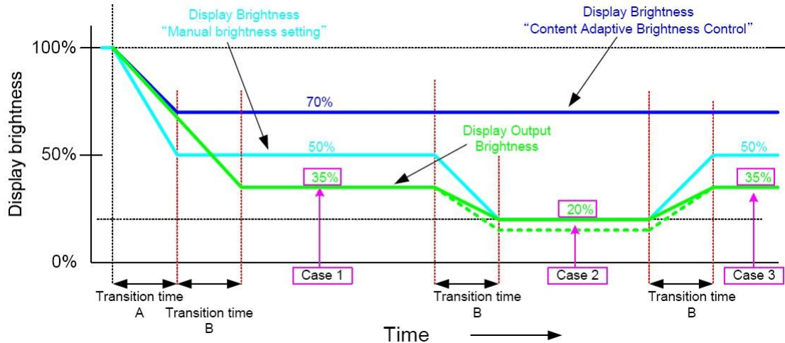
Figure 70. Controlled Display Brightness by LABC and CAB Algorithm
