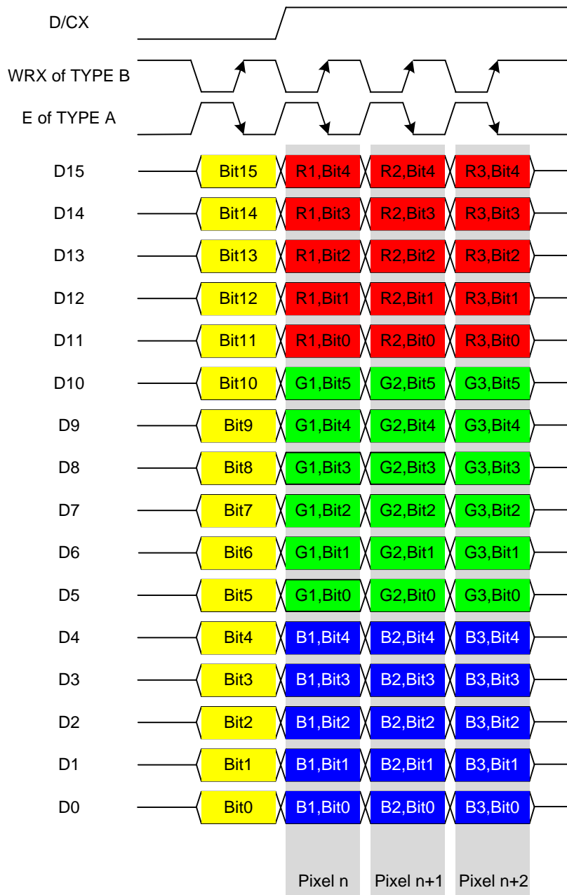
Figure 14. 16-bits/pixel(R 5-bit, G 6-bit, B 5-bit), 65,536 Colors
