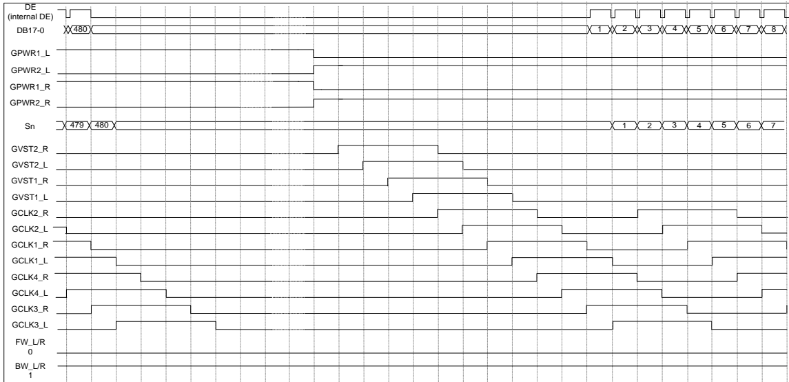
Figure 100. Overlap, 8-phase, backward mode ( FHN=1, SDM=1, FV=1, FVST=0 )
