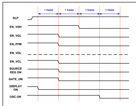
Power OFF STMODE[2:0]=7h
