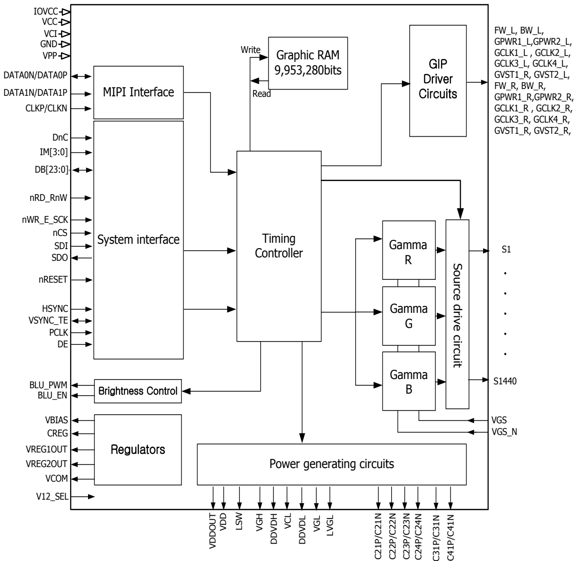
Figure 1. LG4572B Block Diagram
