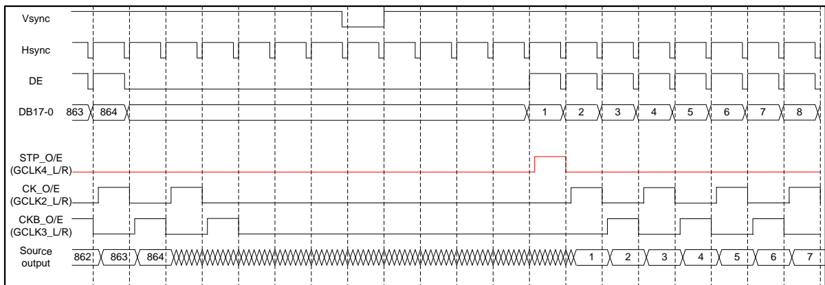
Figure 84. Non-overlap, single scan (FHN=X, ASG=1)
