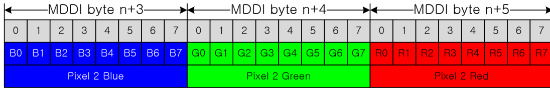
Figure 55. 24bits/pixel(B:8, G:8, R:8) data transfer format
