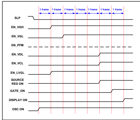
Power ON STMODE[2:0]=1h
