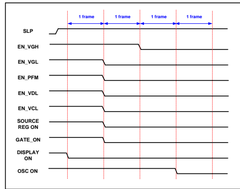
Power OFF STMODE[2:0]=6h
