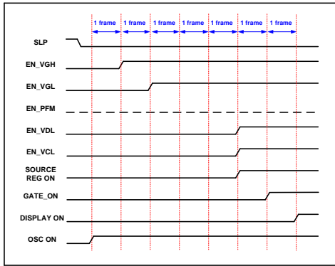
Power ON STMODE[2:0]=5h
