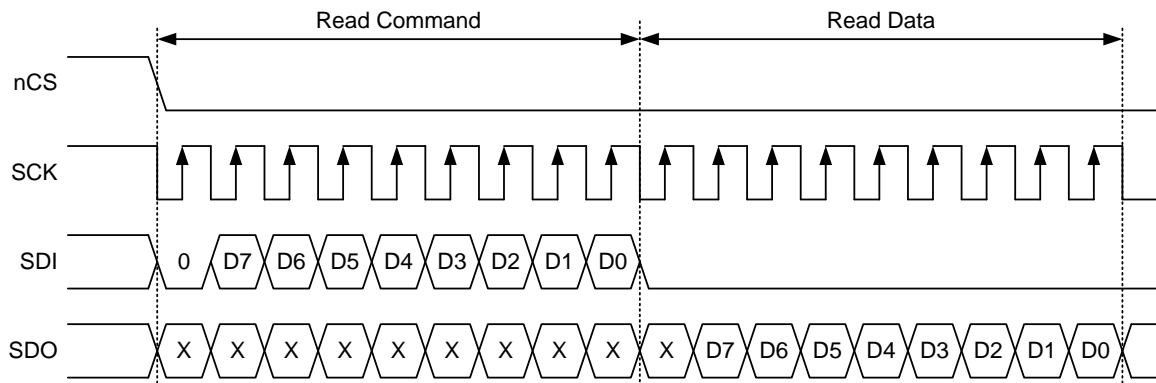
Figure 22. DBI Type C Interface Read Sequence
