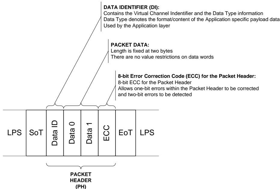
Figure 36. Short Packet Structure
