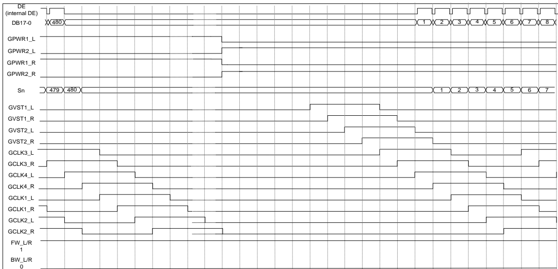
Figure 93. Overlap, 8-phase, forward, advanced DE mode ( FHN=1, SDM=1, FV=0, FVST=1 )
