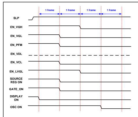
Power OFF STMODE[2:0]=3h
