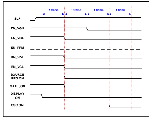
Power OFF STMODE[2:0]=5h
